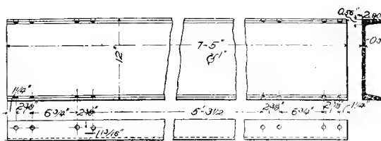
Figs. 4661-4663. Spring-plank Channel iron (1).
